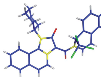
Figure 3. View of the X-ray crystal structure of 5p .
