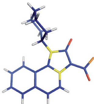
Figure 1. View of the X-ray crystal structure of 5a .
